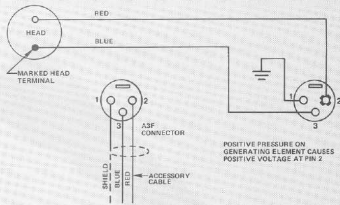
FIGURE 2 – Wiring Diagram
